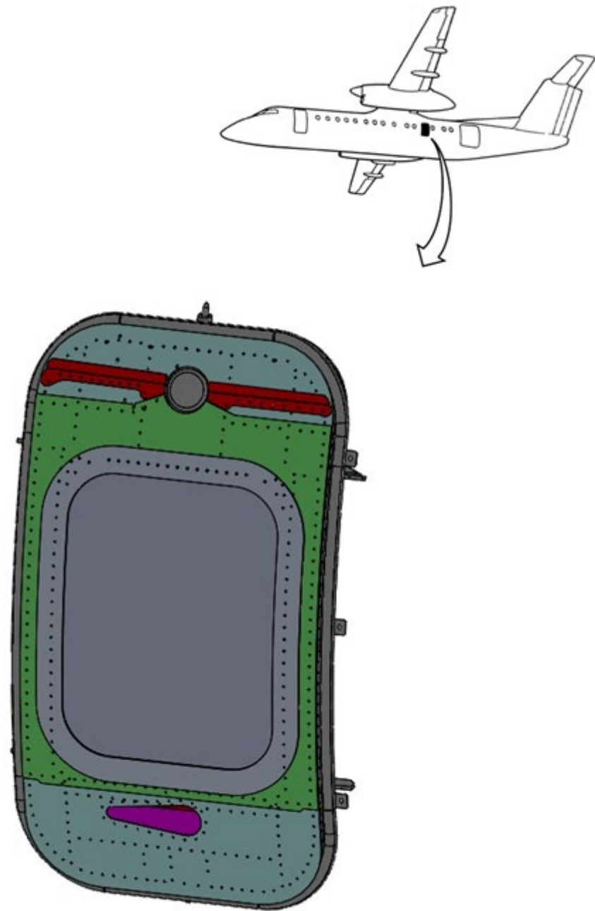
Figure 1: Observer Window Installation (1 per side in existing emergency exit doors)
